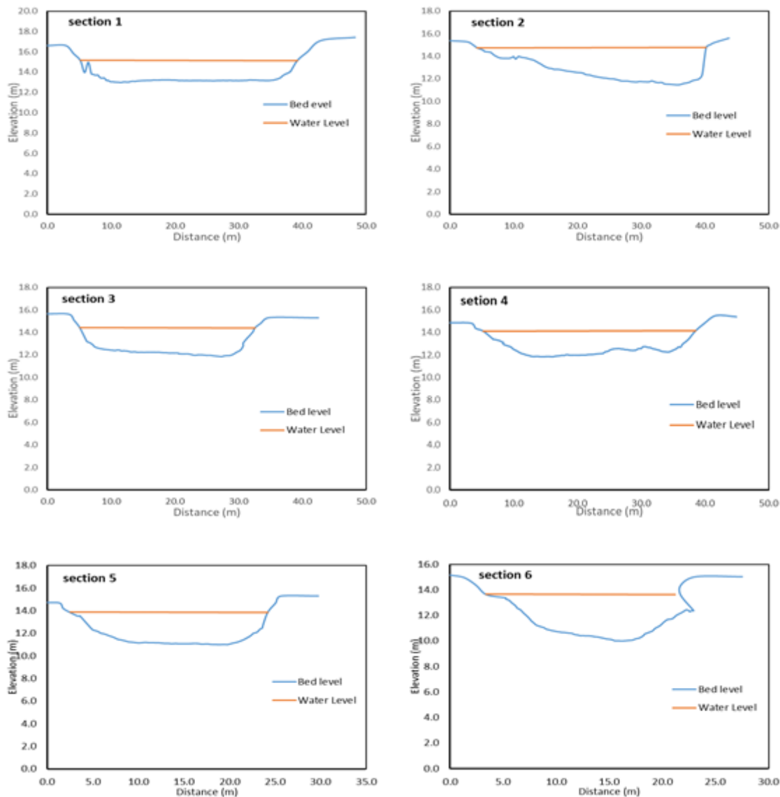
Figure 3: bathymetric survey of the six cross sections provided by (DRI-NWRC)
