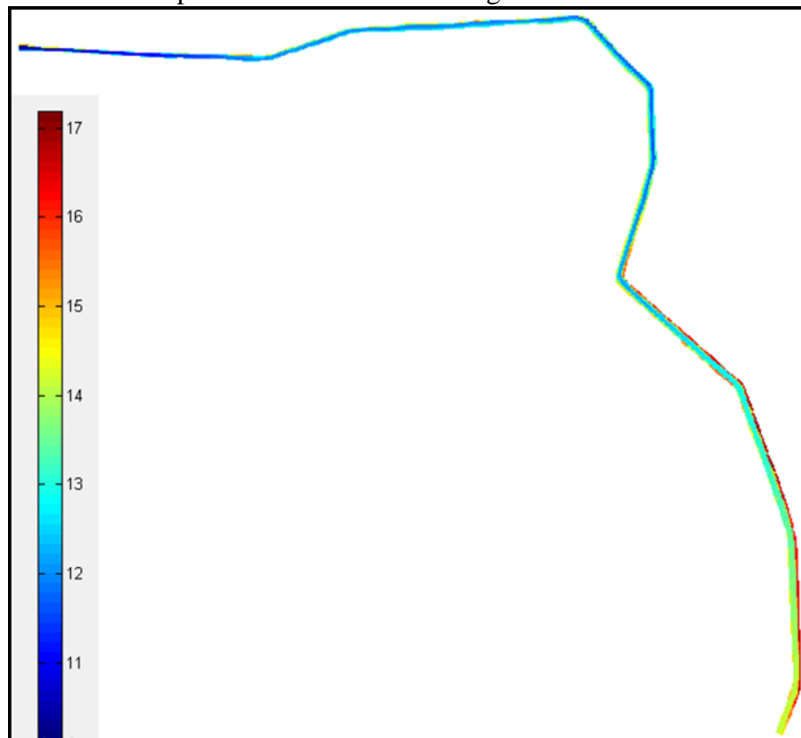
Figure 4: Delft3D showing bed level for the GAWWTP drainage canal
