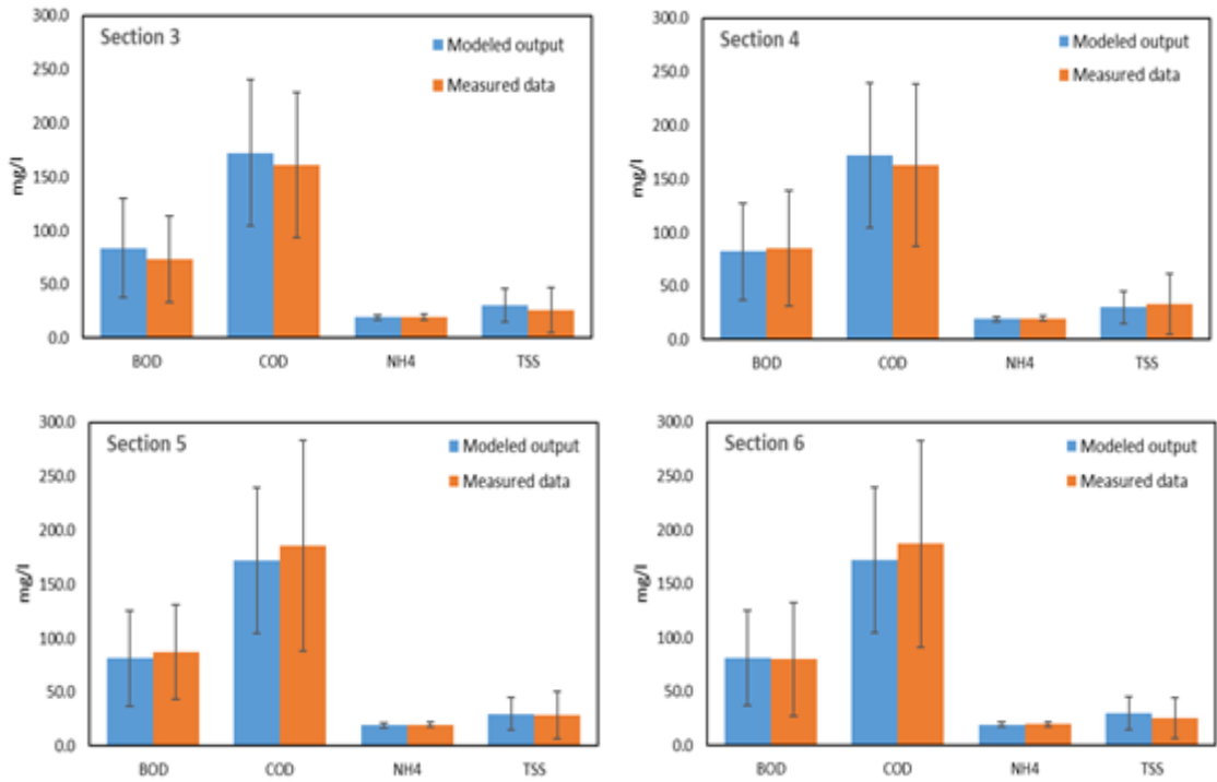
Figure 6: Average values and standard deviations of BOD5, COD, NH4-N and TSS at six sections along the drain
