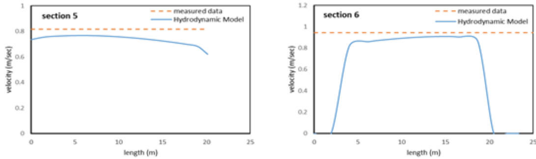
Figure 5: Comparison between the depth average velocity at the field and the model results for the six sections of the study area
