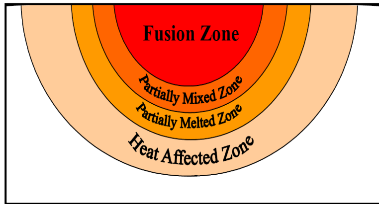
Fig.6 Schematic illustrates the five distinct microstructural zones that exist in dissimilar welds [4].
