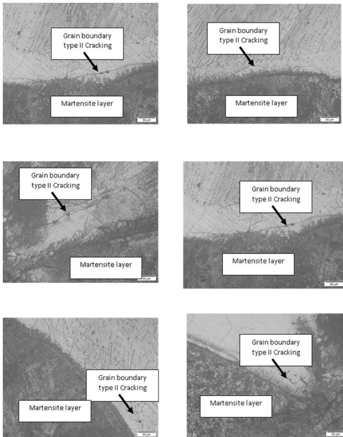
Fig.7 Microstructures at the interface between the weld metal of 316L layer and deposited carbon steel layer that shows the existence of grain boundary type II cracking at different locations.
