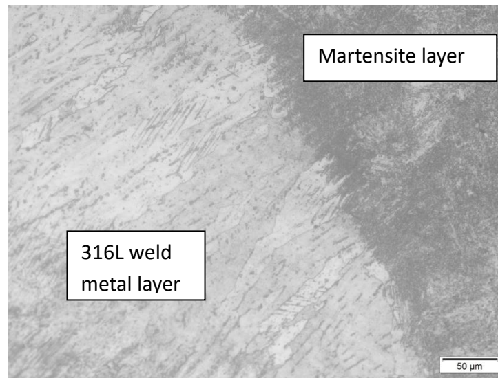
Fig. 9 Microstructure at the interface of the welded joint with deposition of stainless steel on carbon steel weld metal
